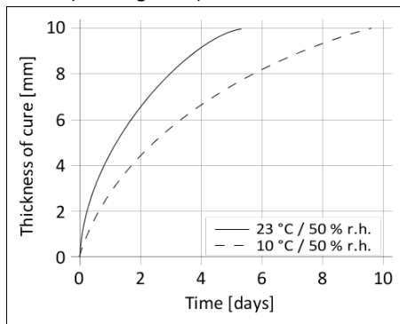
Diagram 1: Curing speed for Sikaflex®-221 LV
