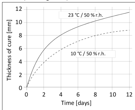
Diagram 1: Curing speed Sikaflex®-221i
